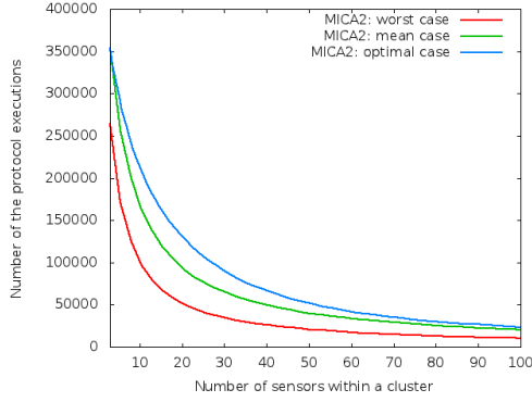
FIG. 2. Performance of EAGDH on MICA2 platform
