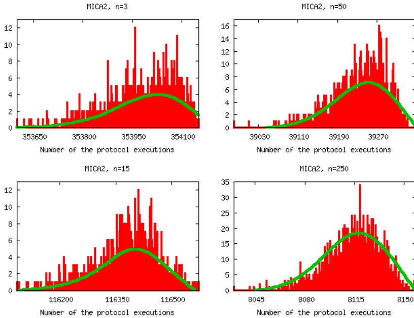
FIG. 6. Histograms of simulations for MICA2
