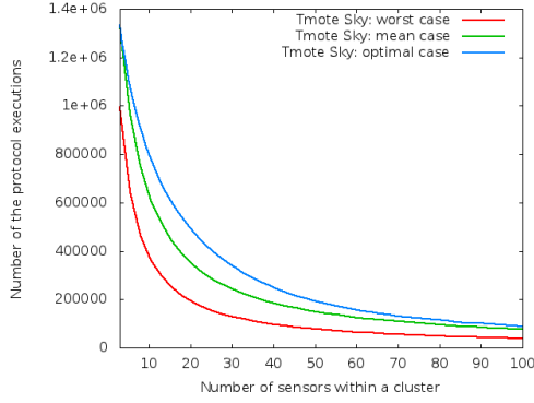
FIG. 3. Performance of EAGDH on Tmote Sky platform
