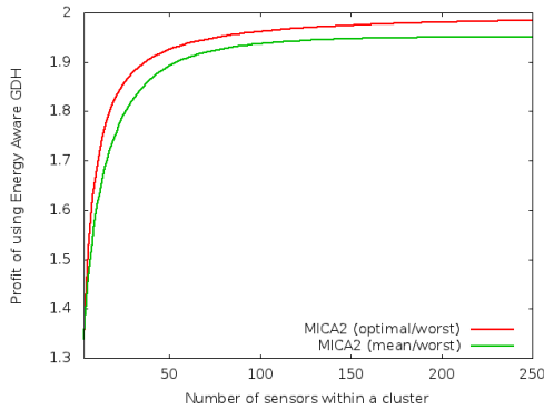
FIG. 4. Profits achieved on MICA2 platform
