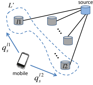
Fig. 1. The proactive caching problem involves selecting, based on the mobile transition probabilities, the set L' of caches to proactively cache object s , in order to achieve (1) while satisfying (2). In the proposed scheme the decision to proactively prefetch a data object is taken independently for each cache.
