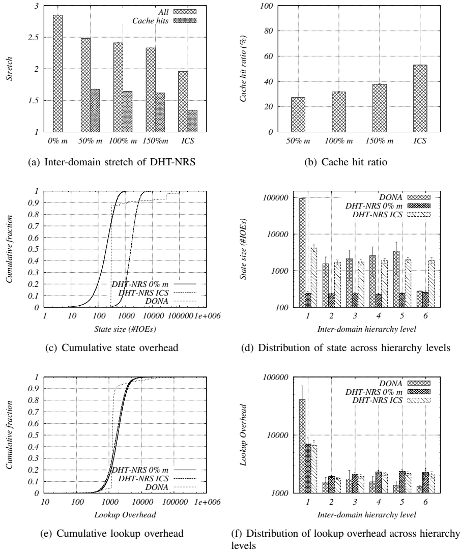
Fig. 2. Performance evaluation results: DHT-NRS vs. DONA
