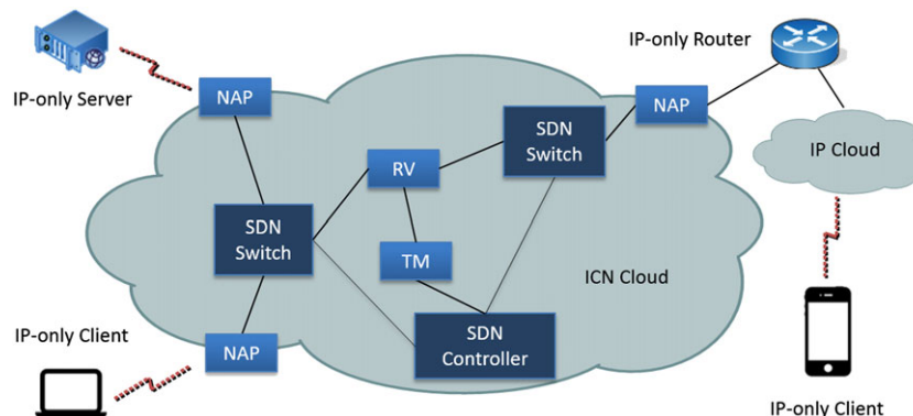
FIGURE 1 The POINT architecture
