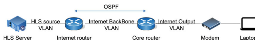
FIGURE 3 PrimeTel's HLS logical network topology
