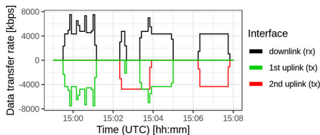
FIGURE 13 Effect of link failover with IPTV over IP
