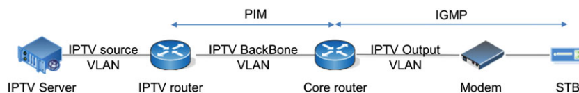
FIGURE 2 PrimeTel's IPTV logical network topology
