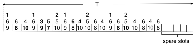
Figure 2: Alternative way to schedule maximal compatible link sets over the TDMA frame for the example of Fig. 1 in line with SDN control paths when node 1 is the SDN Controller. Numbers in bold mark SDN control paths, e.g. , (1) → (8) → (10), (1) → (3) → (5), (6) → (4) → (2), (9) → (7) → (2)).
