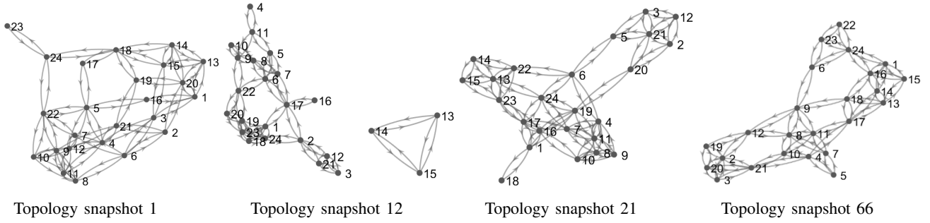
Figure 3: Four network topology snapshots out of the Anglova mobility traces that were used in our numerical evaluation.
