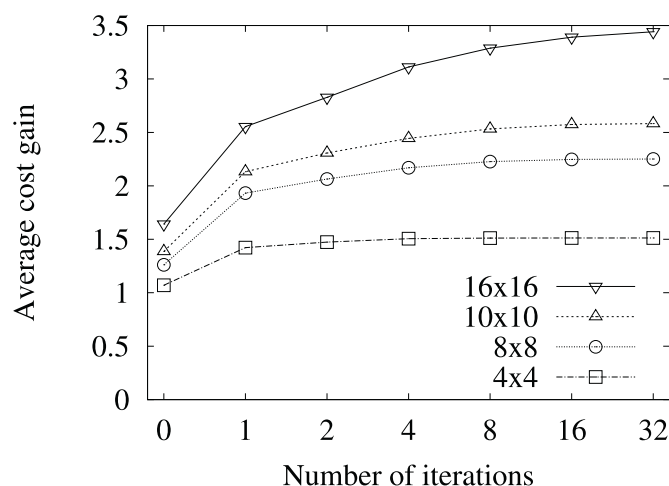
Fig. 8. Average cost gain of DEC-BPn with respect to GR-LQF .
