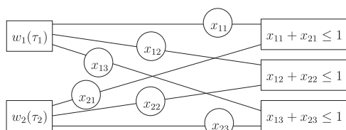
Fig. 2. Factor graph for a 2 \times 3 multicast switch. Circles and rectangles denote variable and function nodes, respectively.
