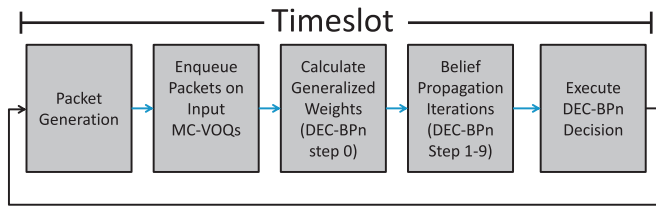
Fig. 11. Temporal sequence of tasks in the datapath of the software router. The third and fourth block corresponds to DEC-BPn scheduler.
