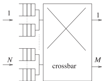
Fig. 1. An N \times M IQ switch with optimal MC-VOQ queueing for multicast traffic.
