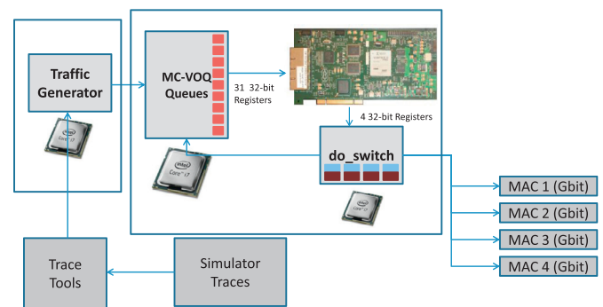
Fig. 13. A hardware/software co-design schematic of DEC-BPn implemented on NetFPGA attached to the PCI bus of an Intel Core i7 motherboard.
