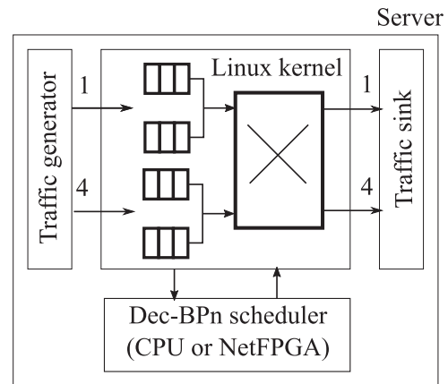
Fig. 12. Implementation of the datapath for 4 \times 4 software router on a Linux server.
