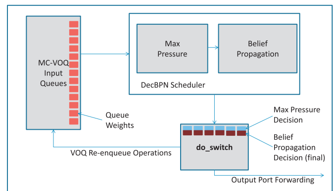
Fig. 10. A high-level schematic of DEC-BPn scheduler integrated with the forwarding datapath of the software router.
