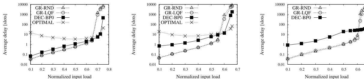
Fig. 7. Average delay under concentrated traffic: (a) Conc-1, (b) Conc-2, (c) Conc-3.
