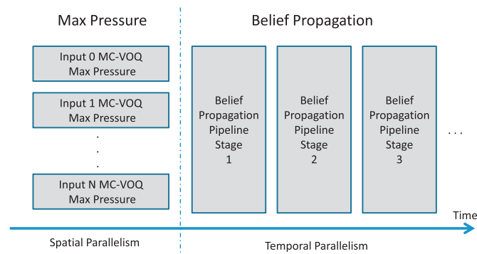
Fig. 9. DEC-BPn processing components, exploiting both temporal and spatial parallelism.
