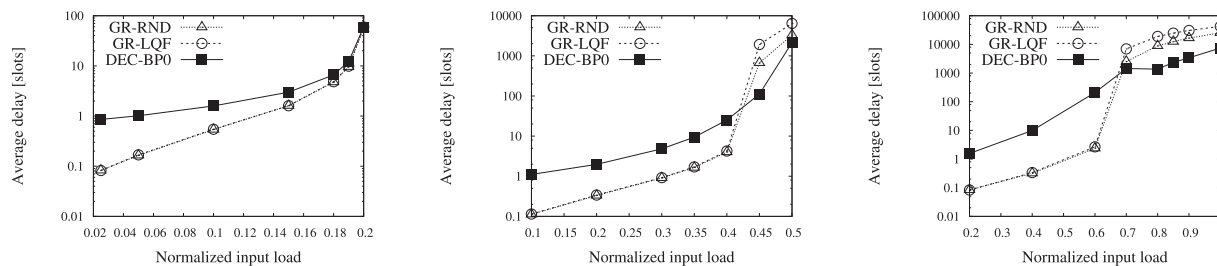
Fig. 6. Average delay under uniform traffic: (a) 10 \times 10 , (b) 4 \times 10 , (c) 2 \times 10 .
