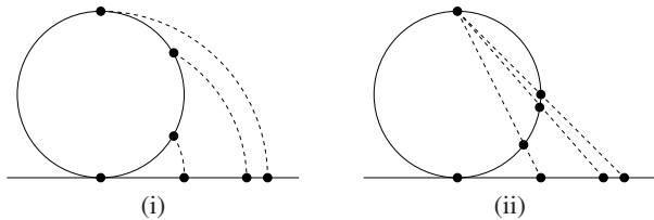
Figure 1. A cross sectional view of the sphere and a plane tangent to it at south pole. (i) Area-preserving map: each point on the sphere (except the north pole) is projected to the plane along a circular arc centered at the point of tangency between the sphere and plane. (ii) Stereographic map: a point p on the plane is mapped to the intersection of the line through p and the north pole with the sphere.
