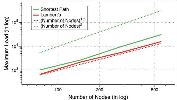
Figure 7. A comparison of maximum load in an L-shaped domain with different routing algorithms. While shortest path have higher maximum load, by Lambert's method, we provide the maximum load closed to \Theta(n\sqrt{n}) .
