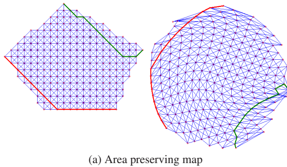
Figure 5. (a) A pentagon with grid nodes and area-preserving map to disk using contours by conformal mapping method (238 nodes, avg degree 7.24.) (b) A comparison of the routing schemes. The X axis represents the node's traffic load on range of loads, while the Y axis shows number of nodes of the corresponding load range. Note the decrease in maximum load on using area-preserving map followed by either azimuthal or stereographic mapping to sphere compared to shortest path routing.
